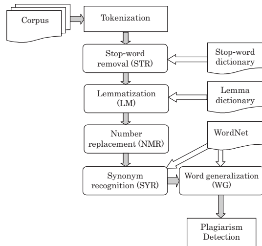
Fig. 1: Text pre-processing scheme
